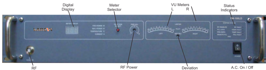
FM-100LD FRONT PANEL CONTROLS AND INDICATORS
