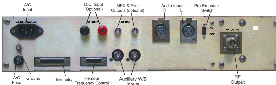
FM-100LD REAR PANEL CONNECTIONS
