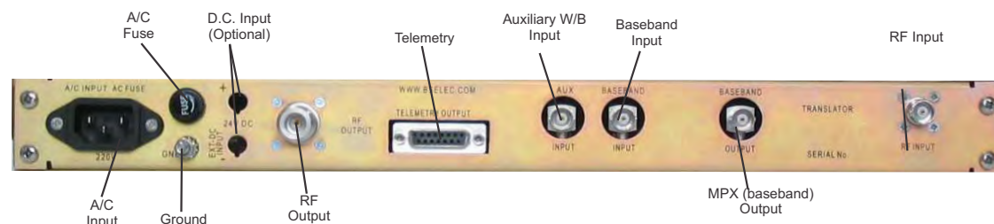
FMT-25 REAR PANEL CONNECTIONS
