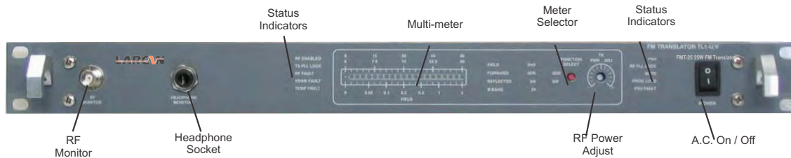
FMT-25 FRONT PANEL CONTROLS AND INDICATORS
