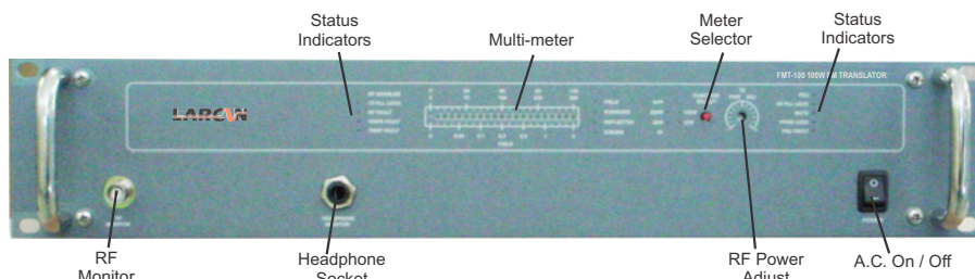
FMT-100 FRONT PANEL CONTROLS AND INDICATORS
