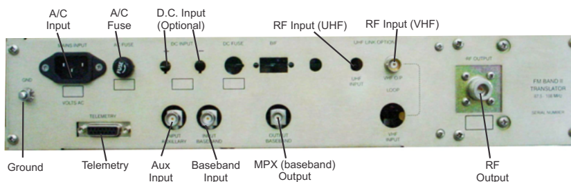
FMT-100 REAR PANEL CONNECTIONS
